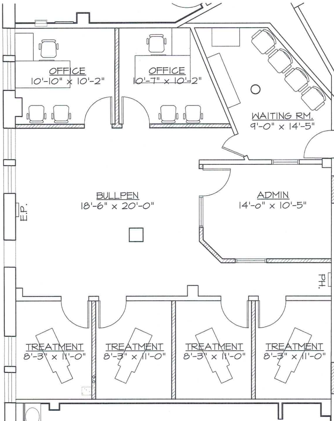
1 PROPOSED PLAN A-1 SCALE: 1/14" = 1'-0"
