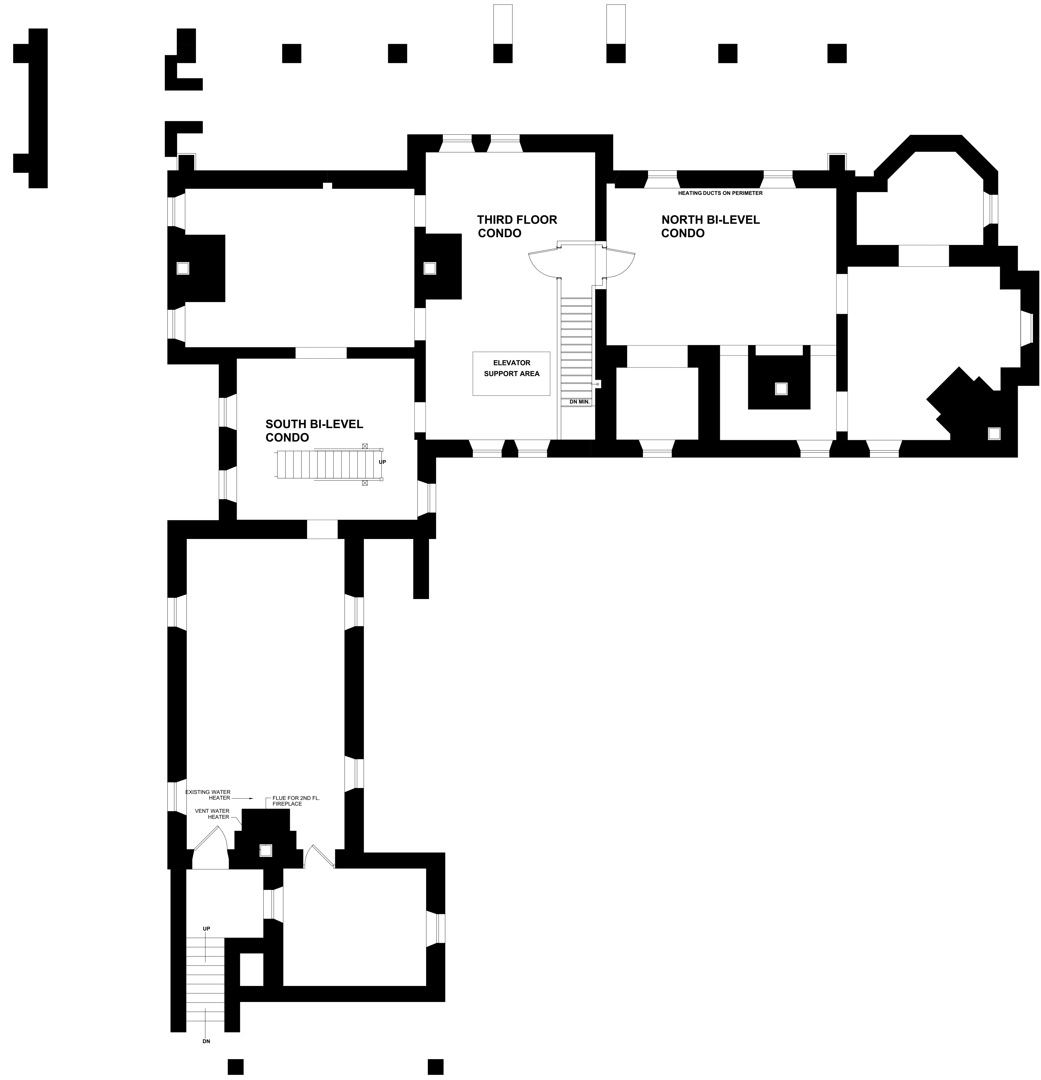
BASEMENT PLAN
