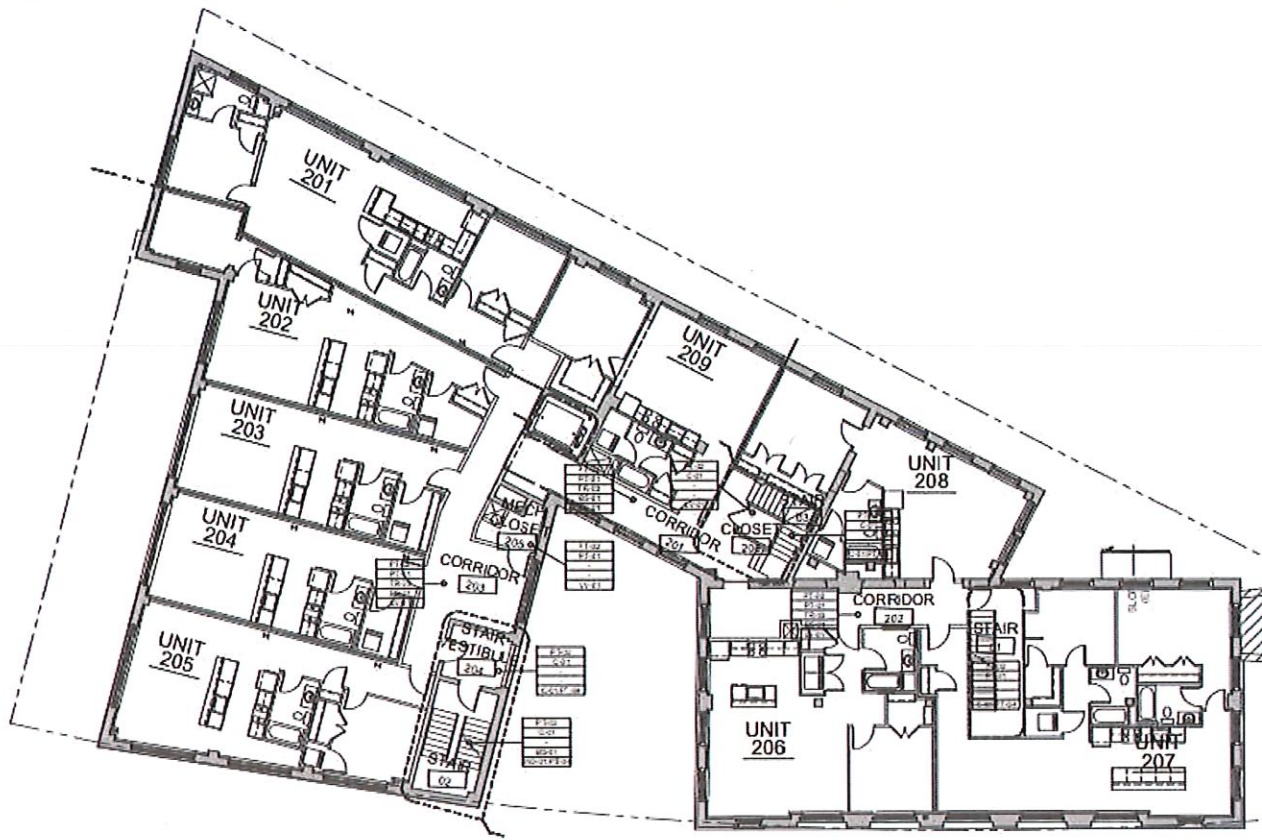
③ SECOND FLOOR FINISH PLAN 1/16" = 1'-0"
