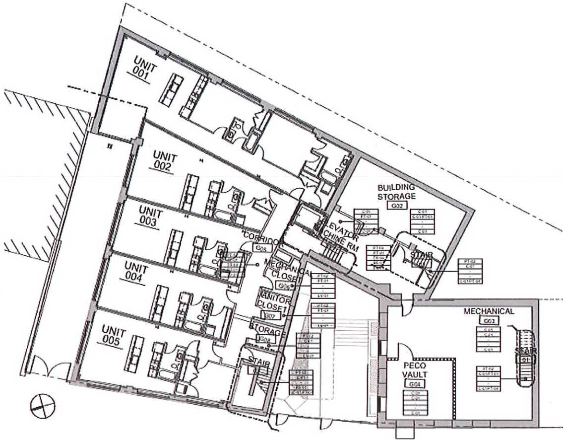
1 GROUND FLOOR FINISH PLAN 1/16" = 1'-0"
